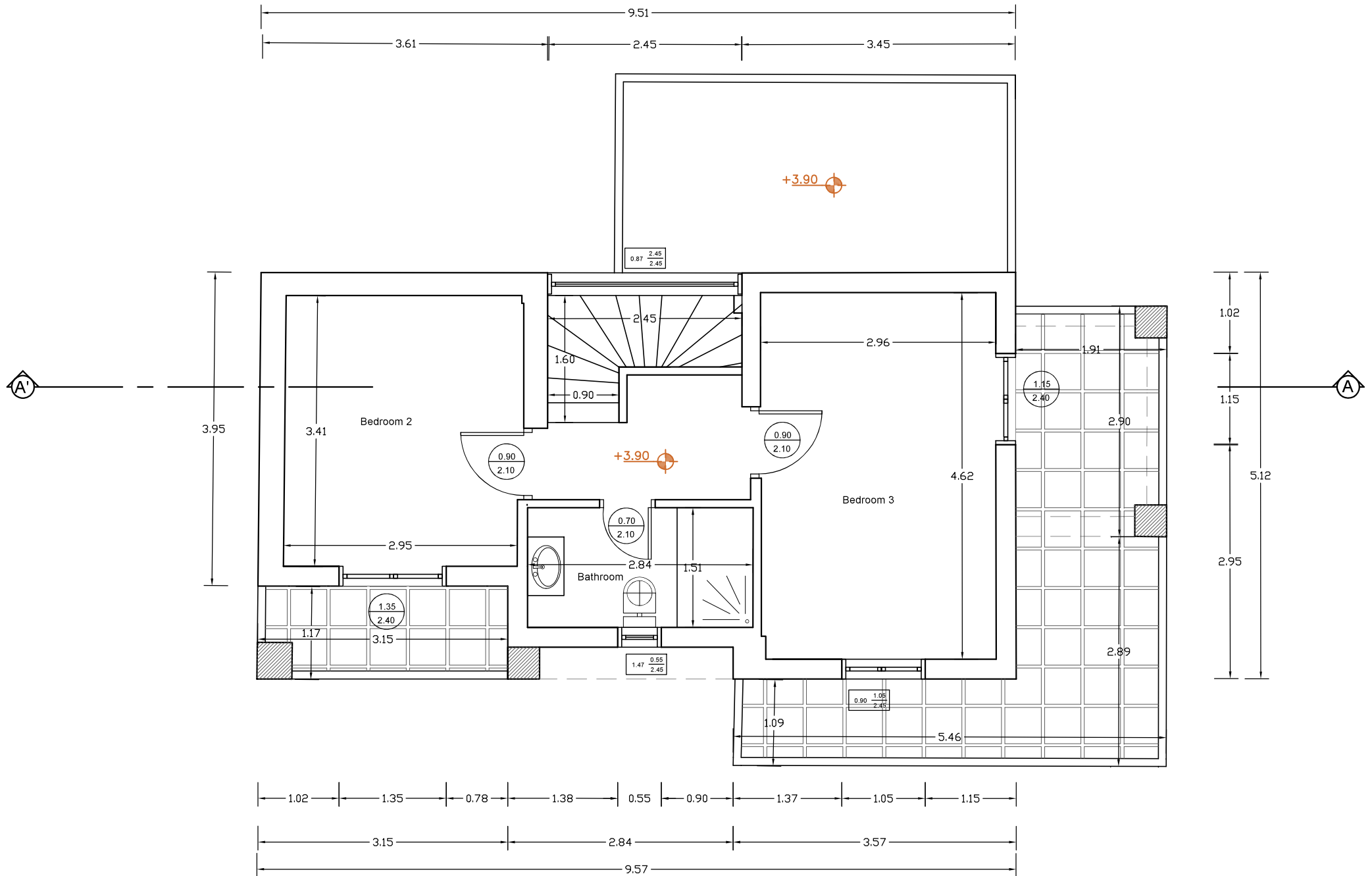
Floor Plan
